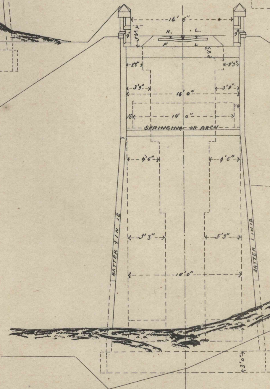
CROSS SECTION.
