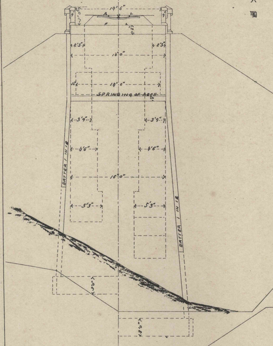
CROSS SECTION.
