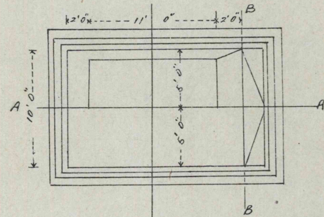
SECTIONAL PLAN AT A A.
