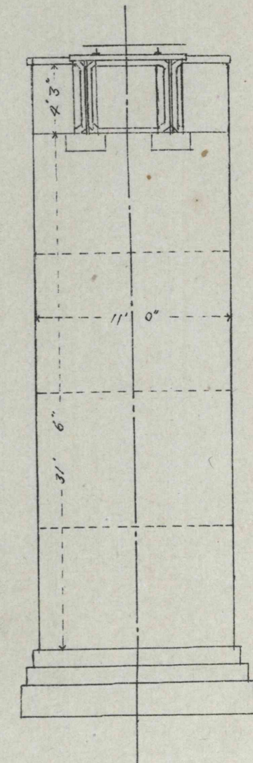
FACE OF RIGHT SIDE ABUTMENT.
