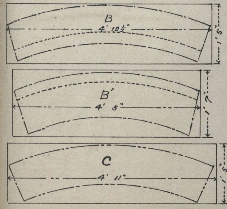
DIAGRAM OF RADIATED PIECES OF WOOD. SHOWING HOW THEY CAN BE CUT FROM SQUARE TIMBERS.
