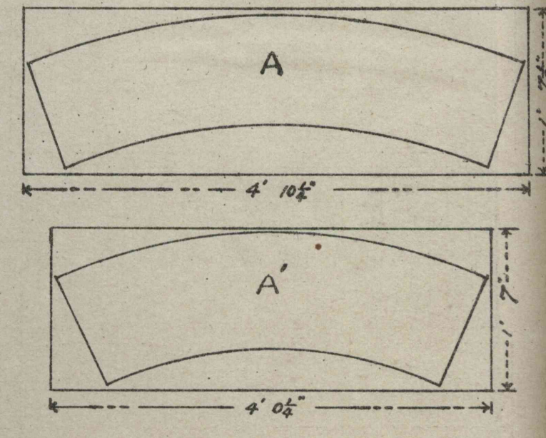
DIAGRAM OF RADIATED PIECES OF WOOD. SHOWING HOW THEY CAN BE CUT FROM SQUARE TIMBERS.
