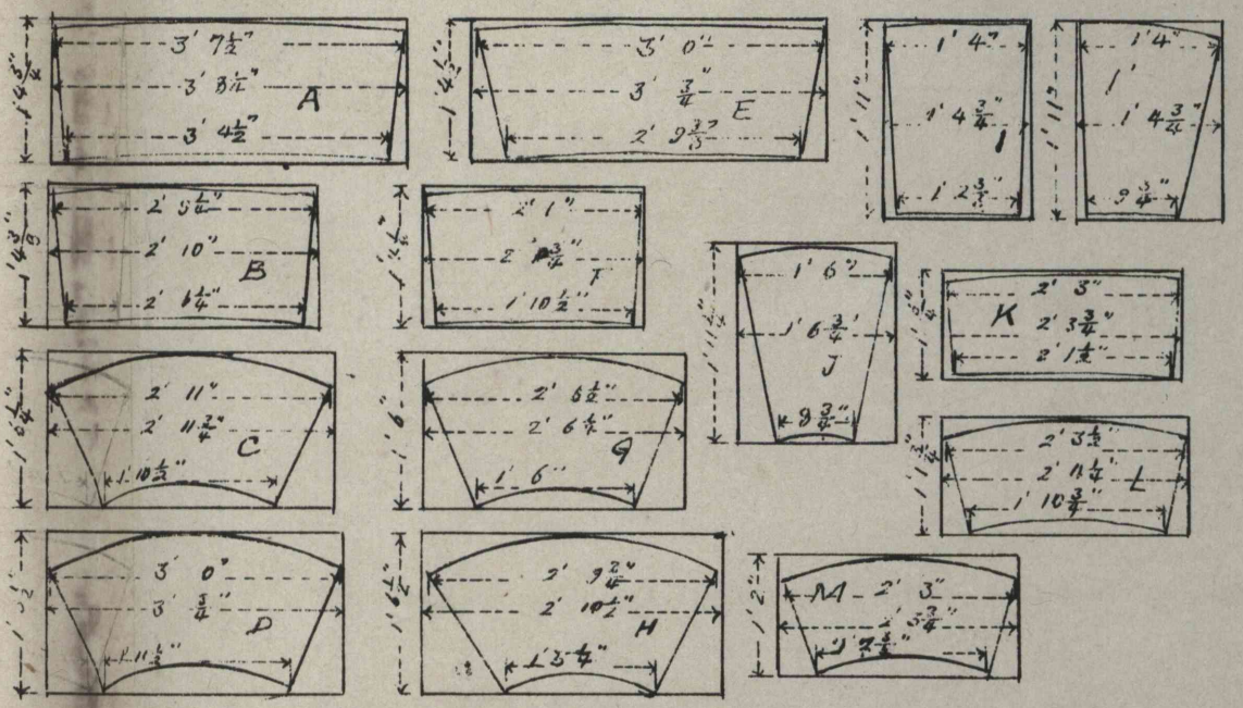
DIAGRAM OF RADIATED PIECES OF WOOD SHEWING HOW THEY CAN BE CUT FROM SQDARE TIMBERS.
