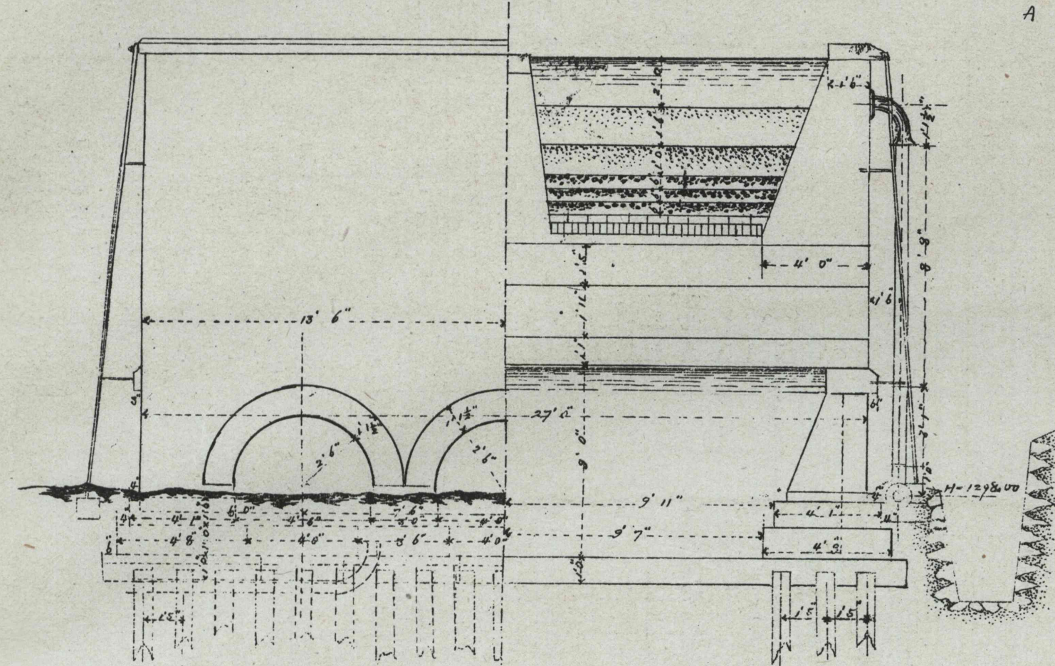
SIDE ELEVATION.
