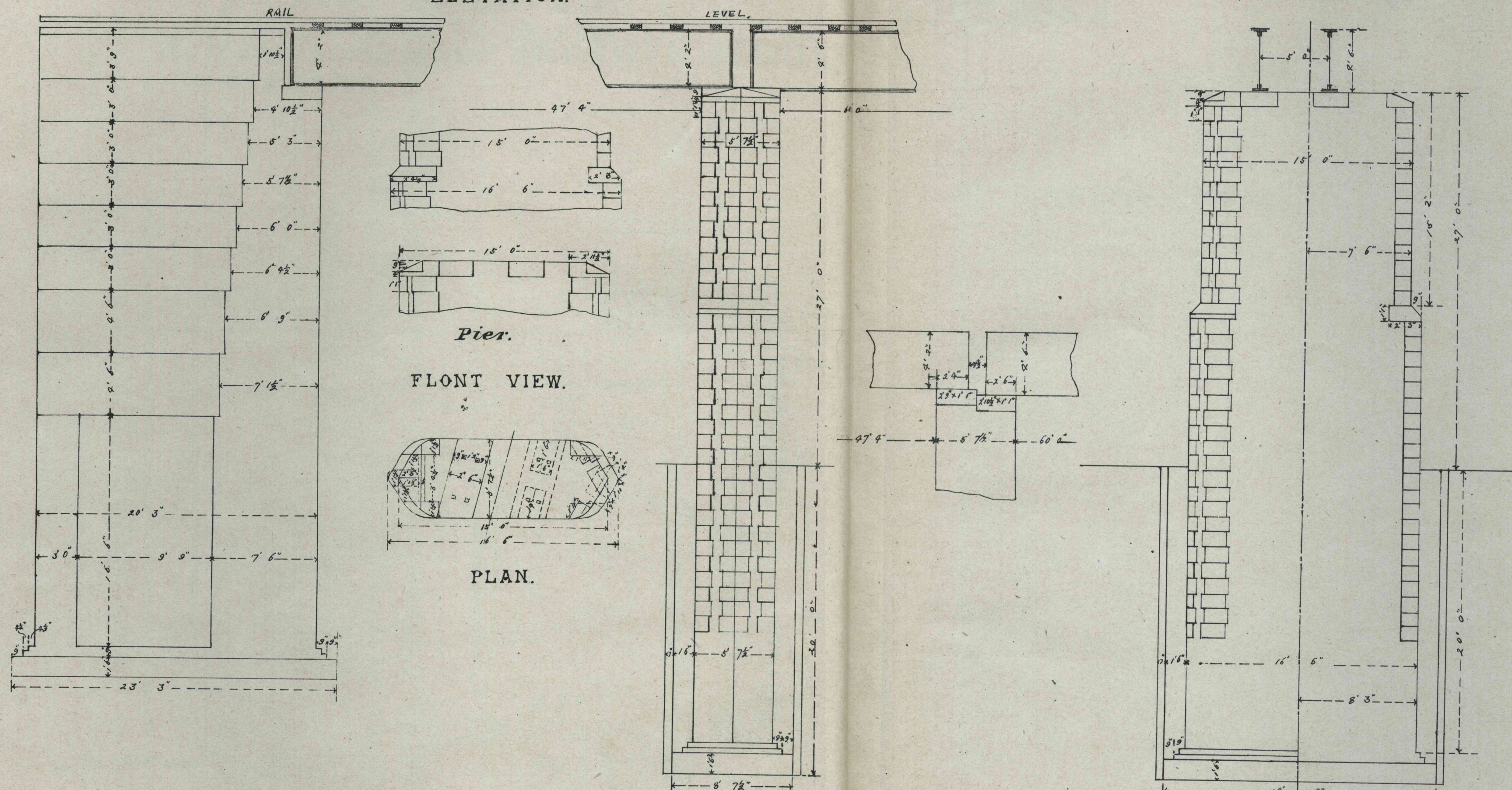
CROSS SECTION.
