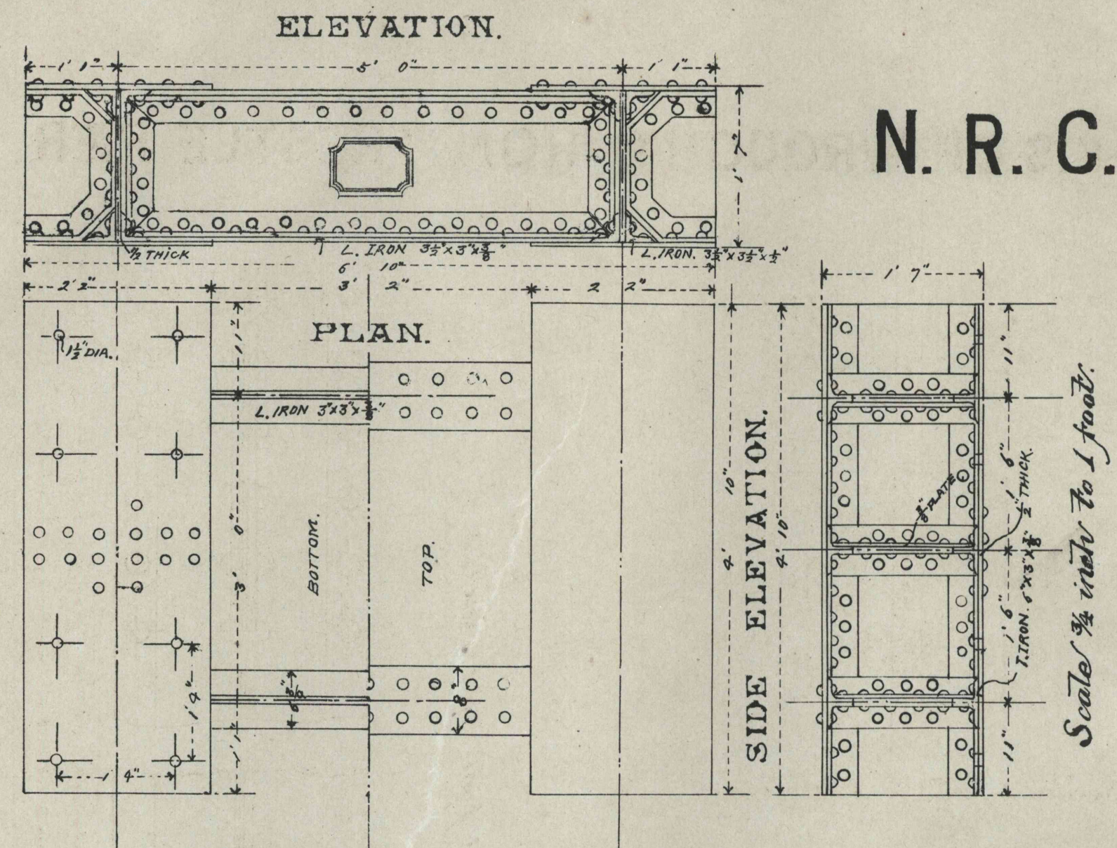
ATTACHMENT OF BASE TO BRICKWORK OR MASONRY.
