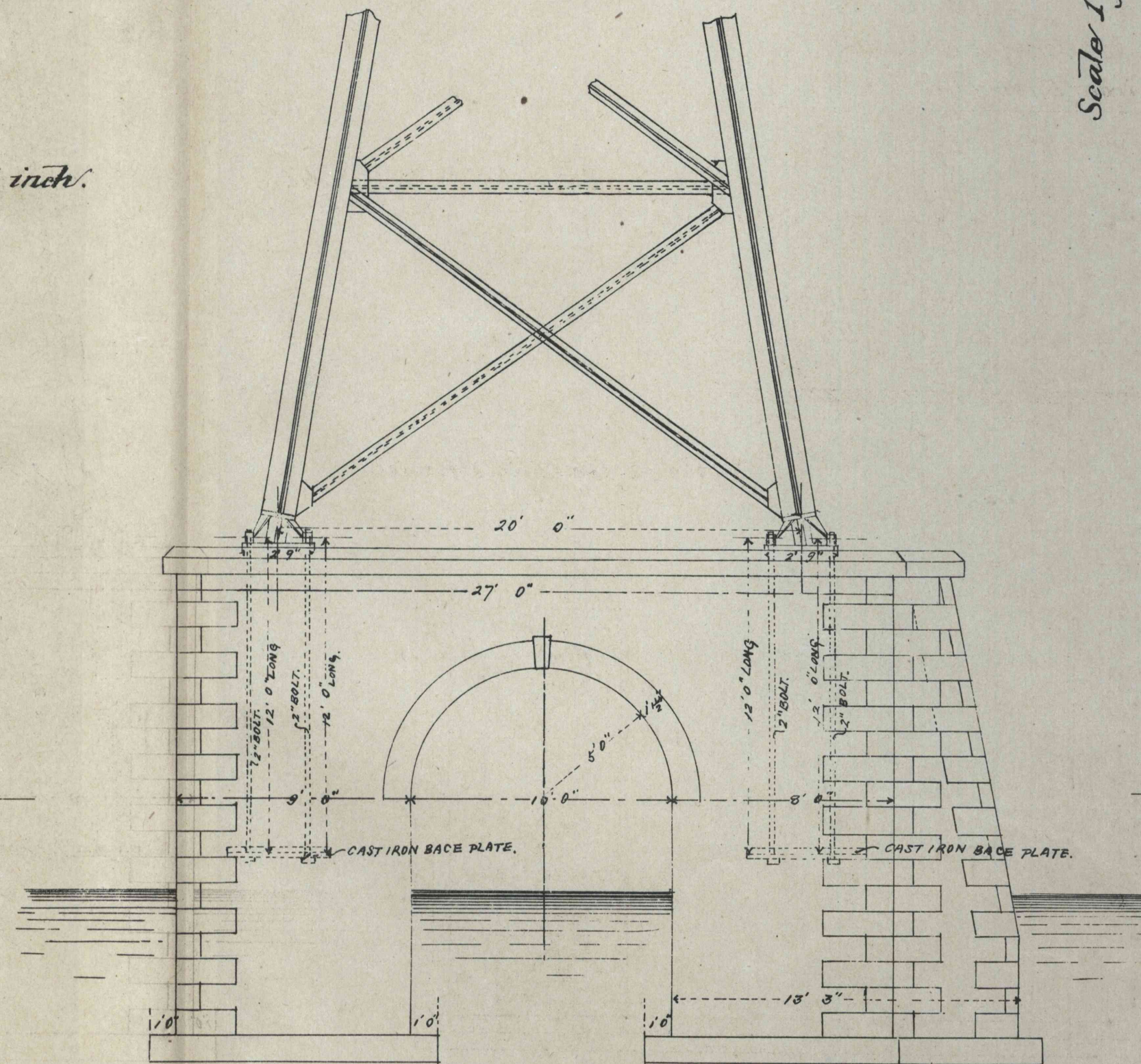
Scale 4 feet to 1 inch.
