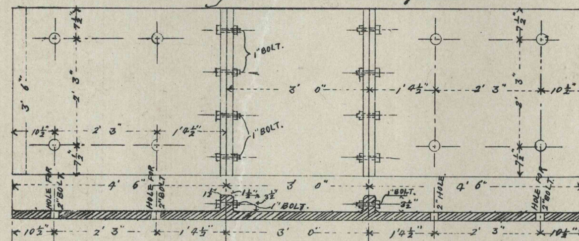
Detail of cast iron base plate.
