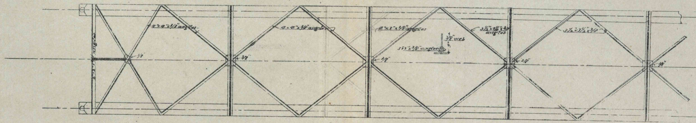
PLAN OF TOP BRACING
