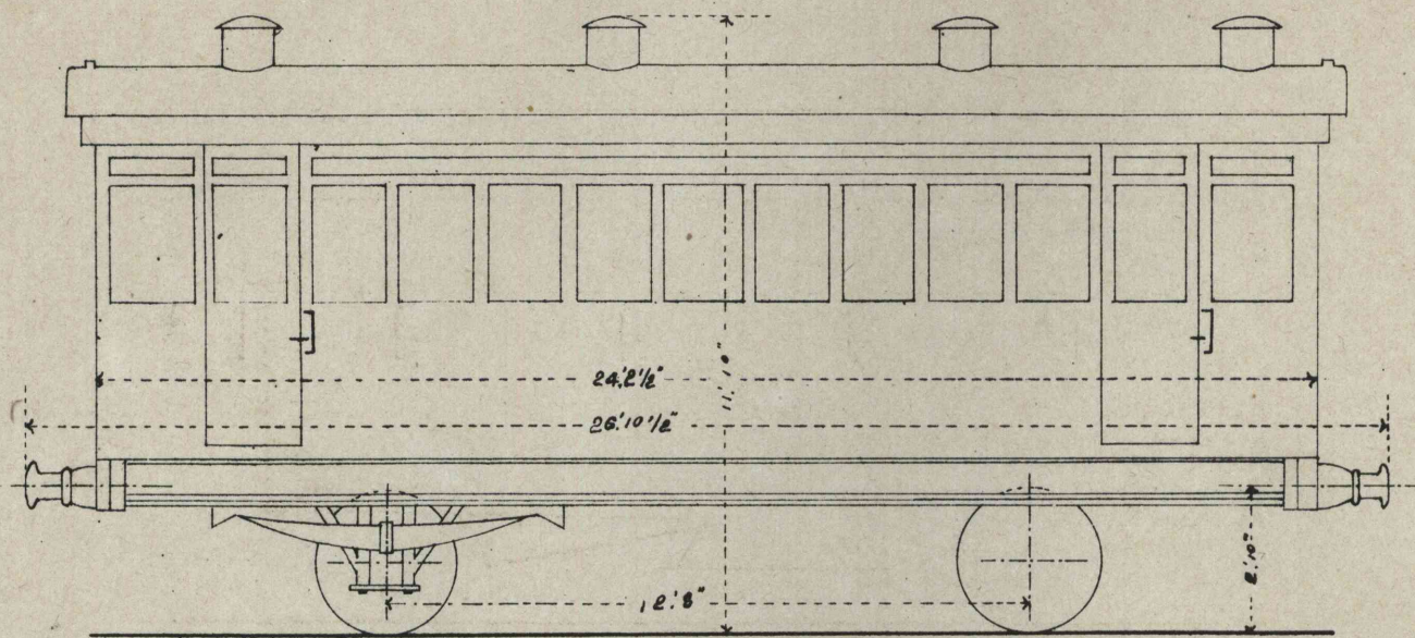
FIRST CLASS CARRIAGE PERSONS 21
