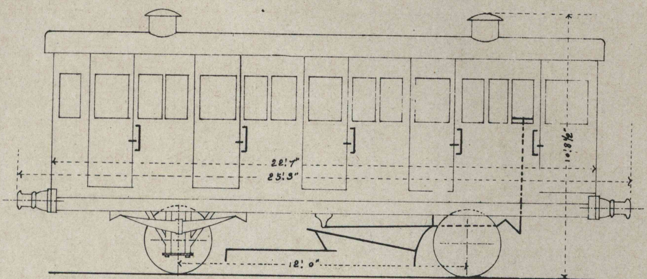
BRAKE VAN AND THIRD CLASS COMPOSITE CARRIAGE
