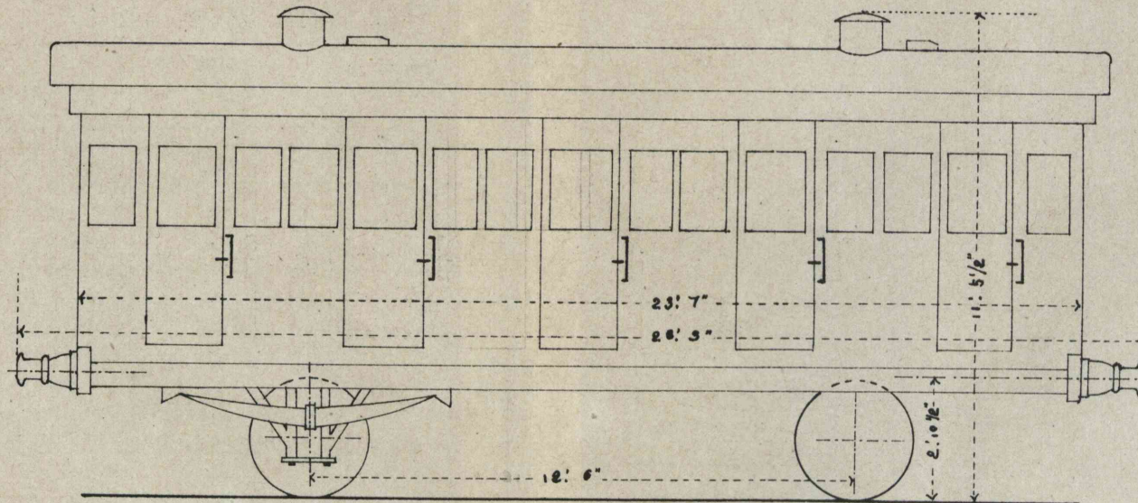
THIRD CLASS CARRIAGE PERSONS 50 23' 7" 25' 11" 0"
