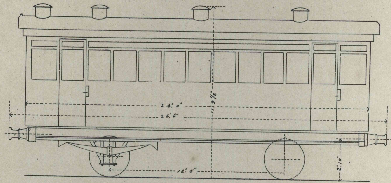
SECOND CLASS CARRIAGE PERSONS 20
