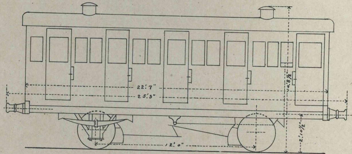
BRAKE VAN AND THIRD CLASS COMPOSITE CARRIAGE PERSONS 48 57' 10 3/4 0/10"
