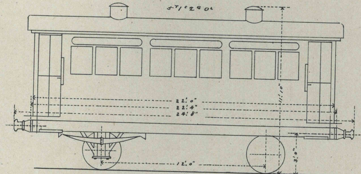
THIRD CLASS CARRIAGE PERSONS 36 57' 2 9/10 0/10"
