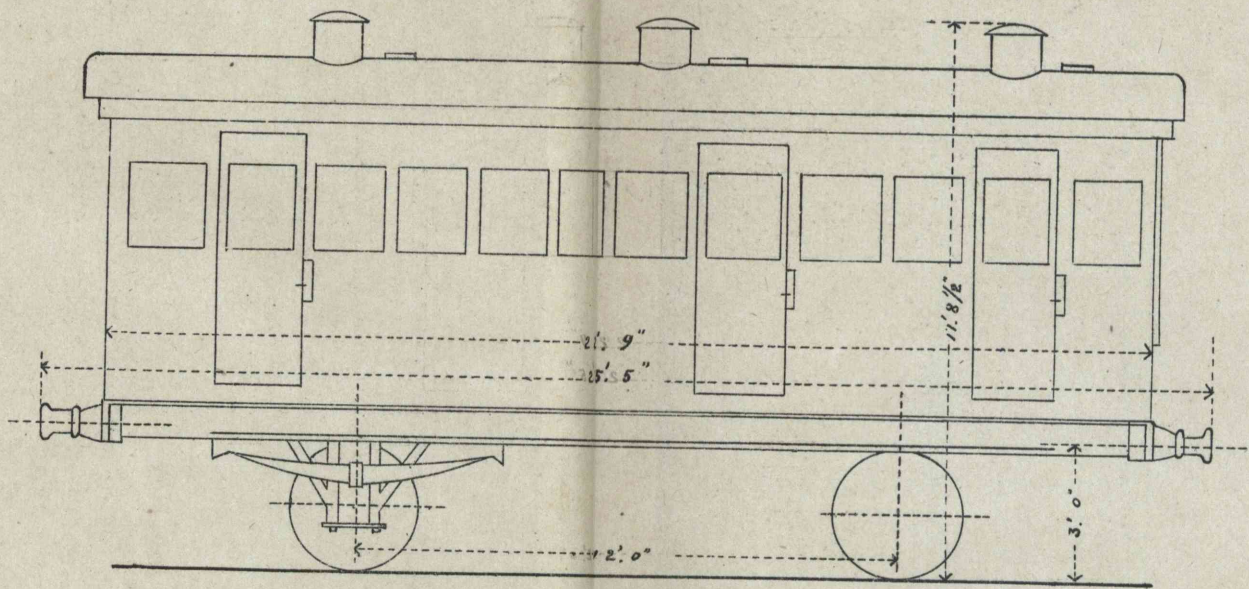
SPECIAL AND SECOND CARRIAGE 67' 10 0/10"
