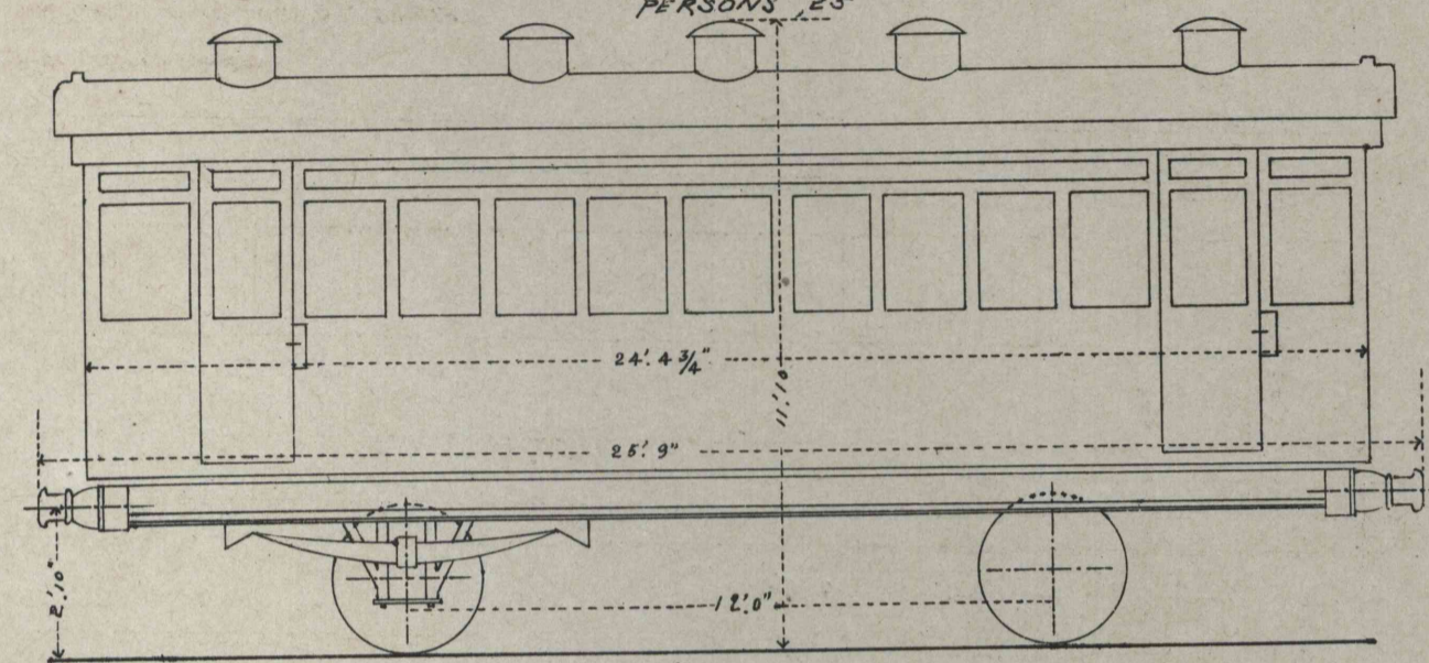
FIRST & SECOND CLASS CARRIAGE PERSONS 25
