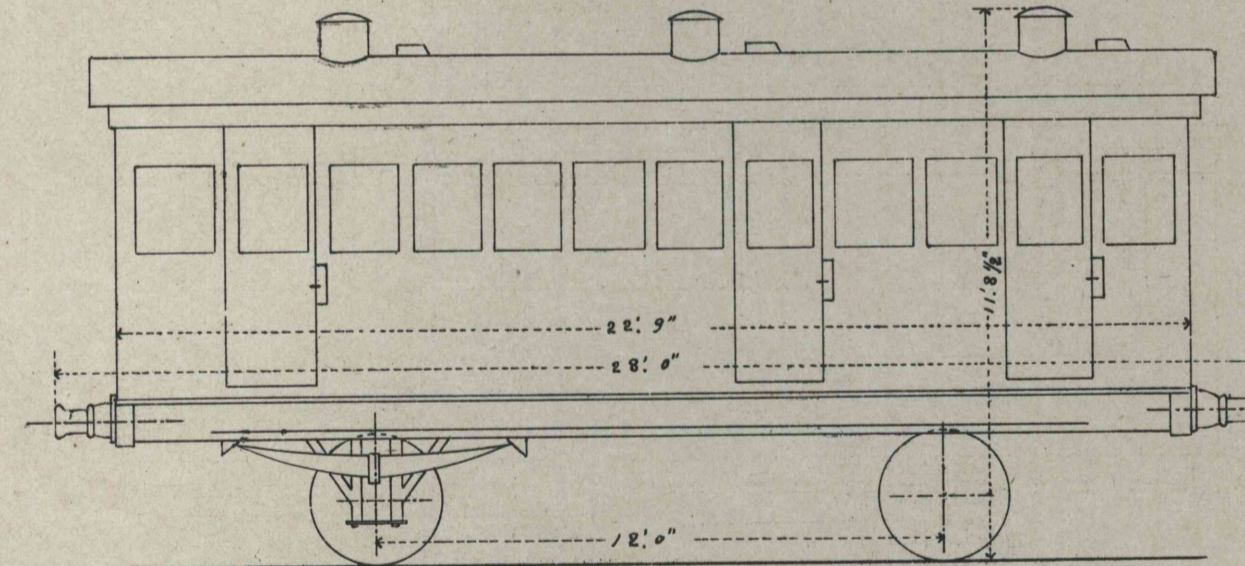
SPECIAL AND SECOND CARRIAGE PERSONS 10
