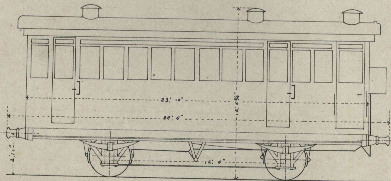
BRAKE VAN & THIRD CLASS CARRIAGE PERSONS 32
