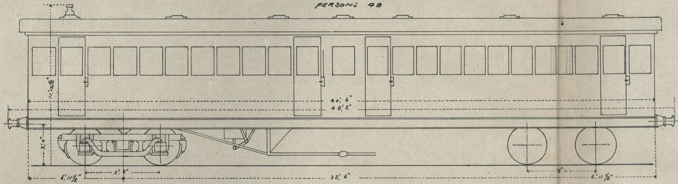
FIRST & SECOND COMPOSITE CARRIAGE PERSONS 48
